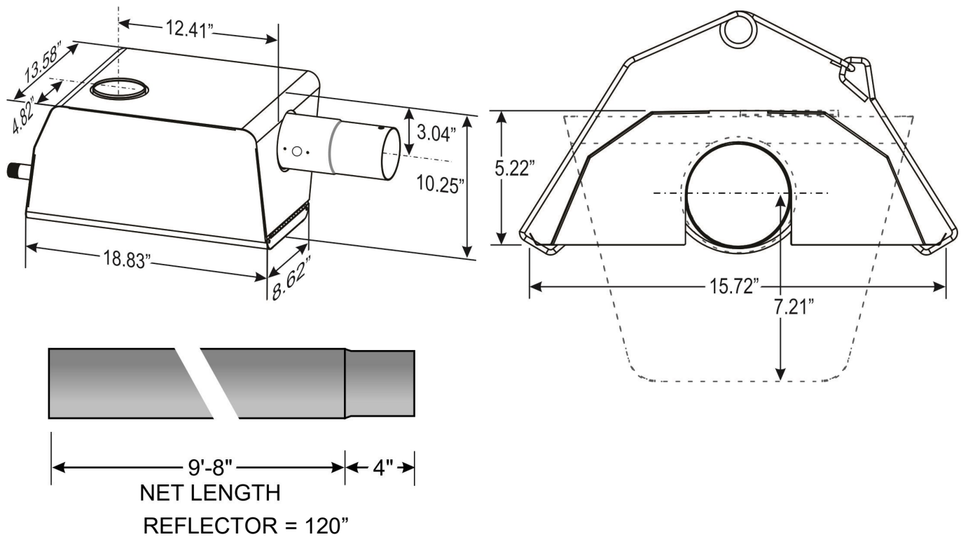
FIGURE 1 HEATER DIMENSIONS
